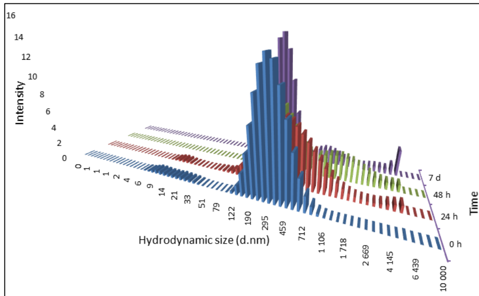
Figure 4. 11- Size distribution of NM-100 for concentration 3.2 \mu\text{g/mL} in cell culture medium at 0, 24, 48 hours and 7 days after dispersion and incubation at 37°C.
