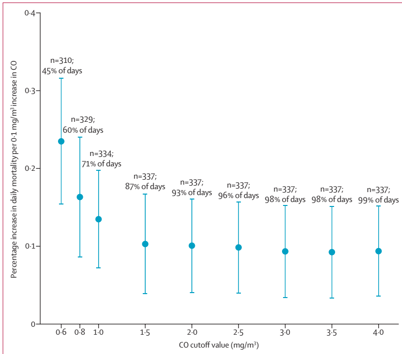
Figure 4: Overall percentage increase in daily mortality per 0.1 mg/m 3 increase in CO (at lag 1 day) by varying cutoff values Cities with at least 365 days of data with CO below the threshold were included. The number of cities (n) and the percentage of observation days included in each threshold analysis are shown. Whiskers show 95% CIs. CO=carbon monoxide.
