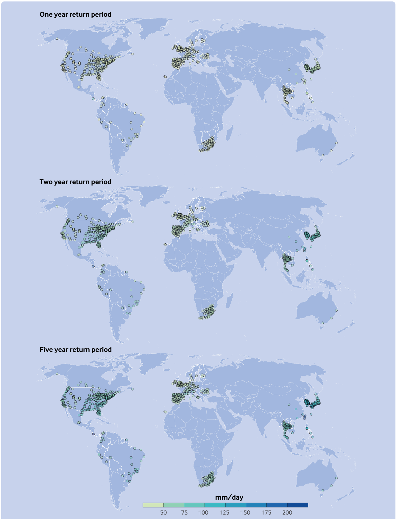
Fig 2 | Daily cumulative thresholds for extreme rainfall events in 645 locations. Analysis used the intensity-duration-frequency model across the three return periods. The return period is the expected average time between occurrences of an extreme event of a certain magnitude
