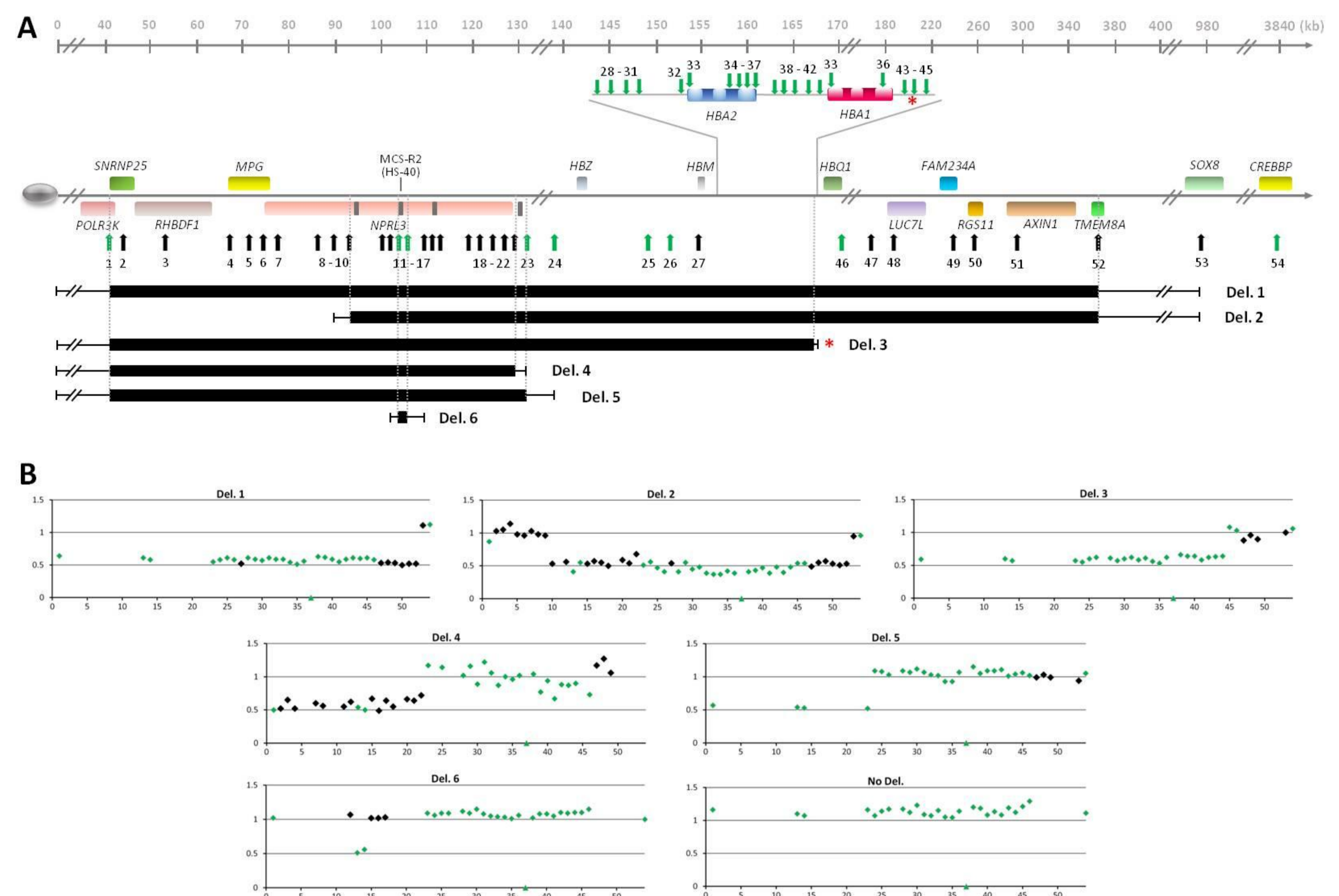
Figure 1. (A) Schematic representation of 4 Mb from the subtelomeric region of chr16p, containing the \alpha -globin gene cluster. MLPA probe hybridization sites are indicated by green and black arrows referring to commercial and synthetic probes, respectively. Each probe is numbered according to their sequential order of chromosomal hybridization. Probe density might not allow individual numbering and therefore probe intervals are shown. Black bars represent deleted DNA sequence as determined by MLPA analysis. Thin lines indicate the region of uncertainty for deletion breakpoints. The oval shape represents the telomere. MCS-Rs are represented by vertical dark grey bars in or nearby NPRL3 gene. (B) MLPA probe ratios (y-axis) were determined by comparison of their signal quantification in the studied individuals and in normal controls. MLPA probe numbers are displayed in the x-axis. Deleted sequences present a probe amplification ratio around 0.5 when in heterozygosity and around zero when the target sequence is deleted in both alleles (exceptions include probes nos. 33 and 36 which hybridize in both HBA2 and HBA1 and therefore, ratio can vary by 0.25 fold). Probe no. 37 is amplified only in the presence of Hb Constant Spring ( \blacktriangle ). *Indicates breakpoint location of deletion 3 in the \alpha -globin gene cluster detailed region.
