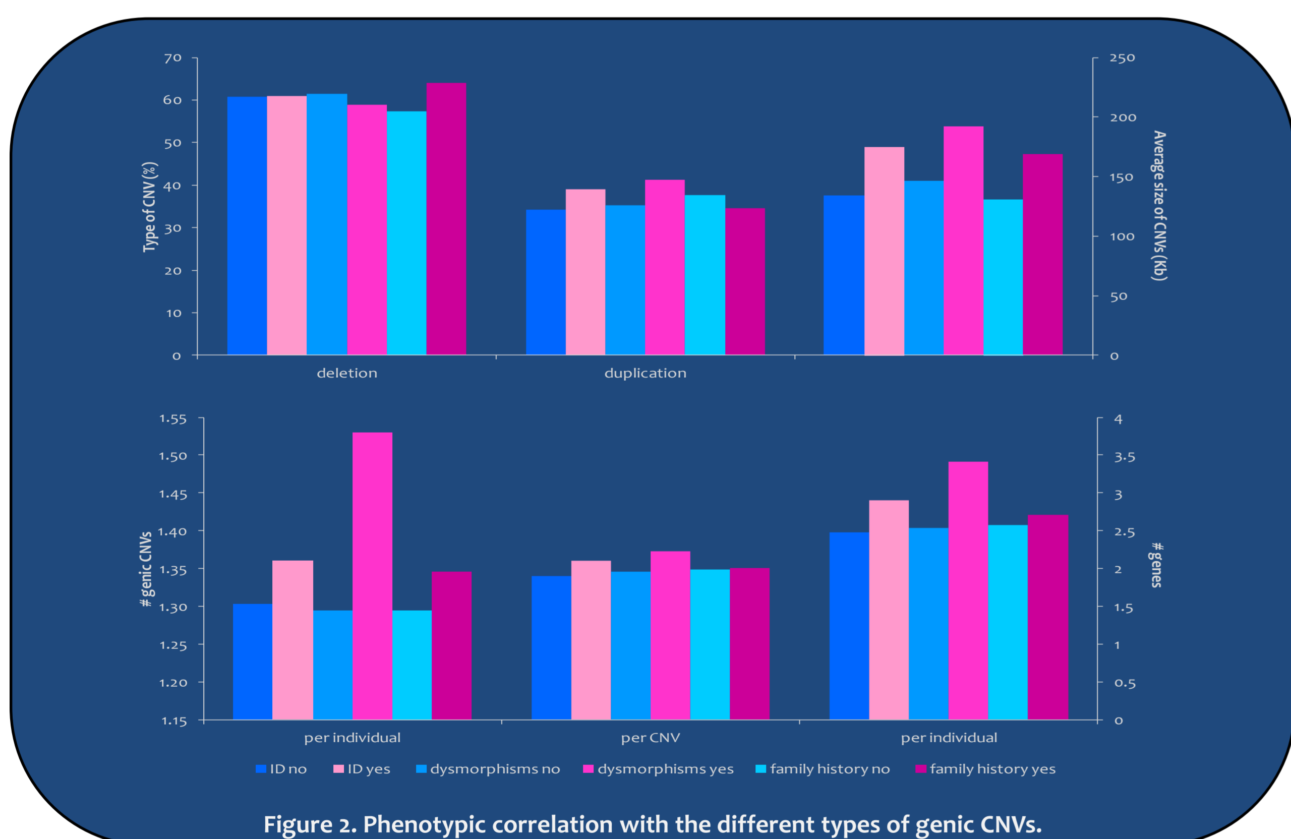
Figure 2. Phenotypic correlation with the different types of genic CNVs.
