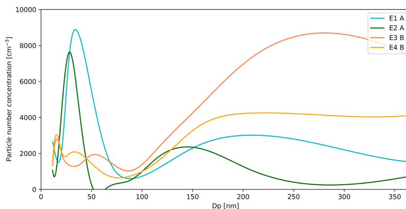
Fig. 4. Particle size distribution for aerosols emitted during the A and B tile cutting experiments. E: Experiment.
