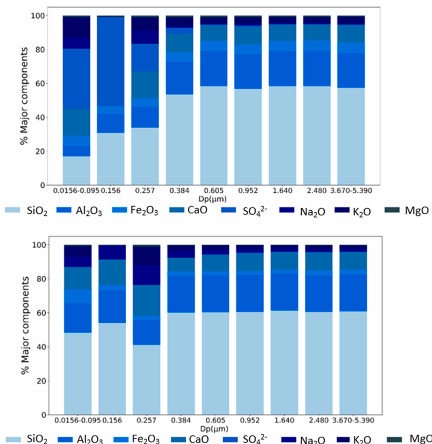
Fig. 5. Size-resolved relative chemical composition of aerosols sampled using an ELPI + impactor (14 stages), on polycarbonate impaction plates. Filters corresponding to 0.0156–0.095 and 3.670–5.390 μm were digested together for ICP analysis, as the sample mass on each individual filter was insufficient for separate analysis. Top: A aerosol release; bottom: B aerosol release.
