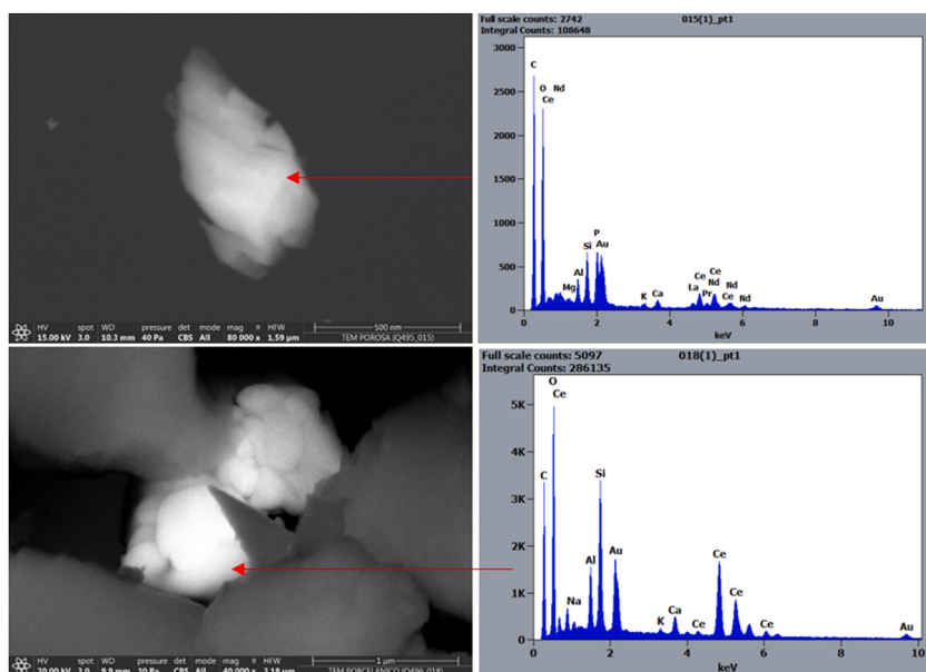
Fig. 7. Ceramic aerosol particles from A (top) and B (bottom) tiles.
