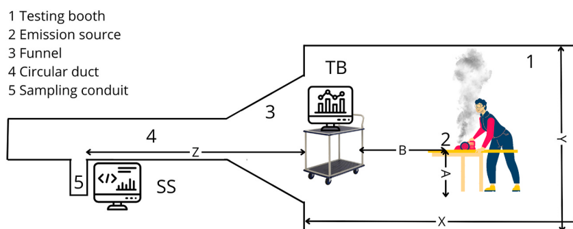
Fig. 1. Testing booth scheme. Dimensions: X = 3\text{m} , Y = 3\text{m} , A = 1\text{m} , B = 0.5\text{m} Z = 3\text{m} .
