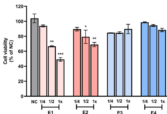
Fig. 8. Human alveolar epithelial cells viability (% of negative control; NC) after exposure for 24h to PM 2 fractions collected during two independent experiments of rotary dry cutting of tile A (E1 and E2) and tile B (E3 and E4).
