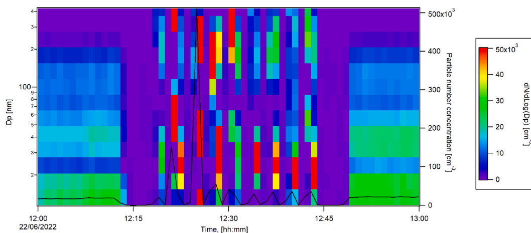
Fig. 3. Nanoparticle release during experiment 1 (Tile A). Particle diameter (Dp) in logarithmic scale.
