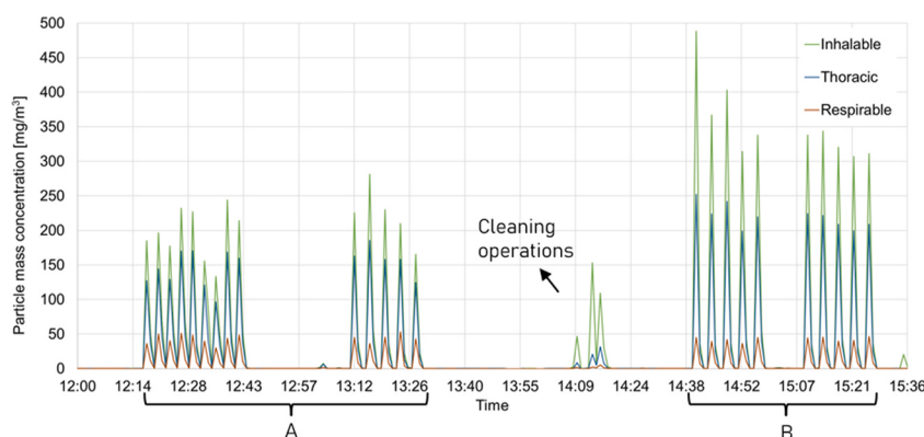
Fig. 2. Particle mass concentrations ( \text{mg}/\text{m}^3 ) recorded in the testing booth during the experiments. Chamber cleaning operations are indicated.
