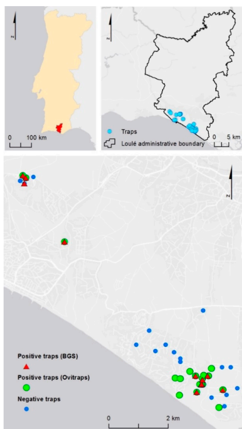
Figure 1. Aedes albopictus monitoring stations in the municipality of Loulé, Algarve, Portugal. Eight BG-sentinel traps baited with BG-lure (BGS, Biogents, Germany) and 36 Ovitrap were used during the study period. Positive traps for Aedes albopictus : red triangles = BGS traps, green dots = Ovitrap.
