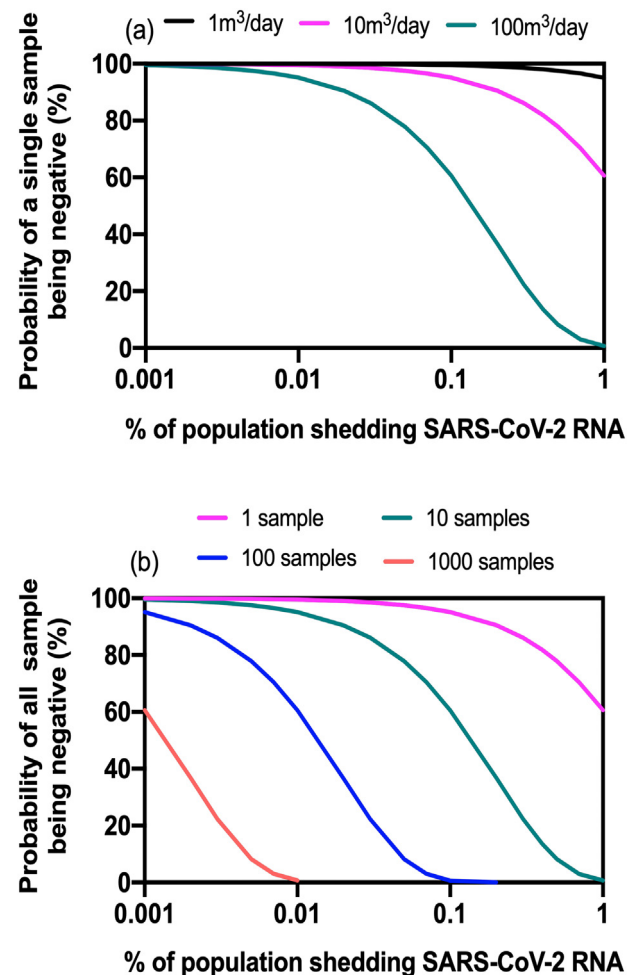
Fig. 3. a: Probability of a single small grab sample (relative to SARS-CoV-2 dispersion volume) being negative, assuming a sewer catchment population of 100,000 people, an average dry weather flow of 0.2 m 3 /person/day, and dispersion volumes of 1 m 3 /day, 10 m 3 /day, or 100 m 3 /day. 3b: Probability of all samples being negative for n = 1, 10, 100 , or 1000 samples.
